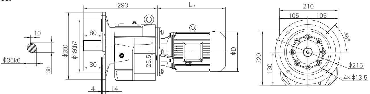
Flange-mounted
