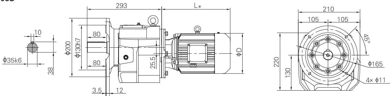
Short flange-mounted
