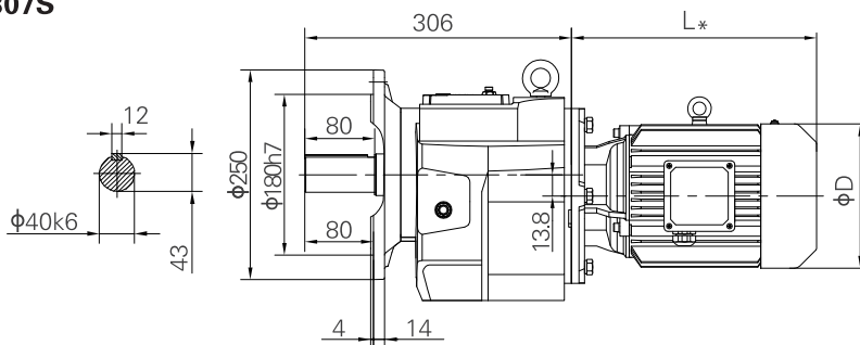
Short flange-mounted
