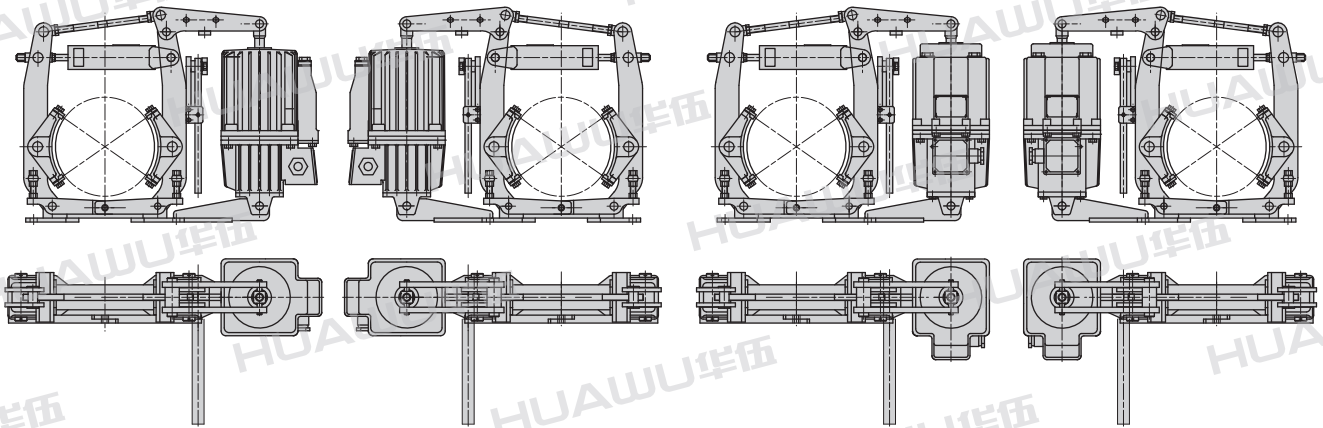
I A型安装 Installation of I A
