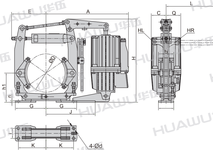
II A型安装 Installation of II A
