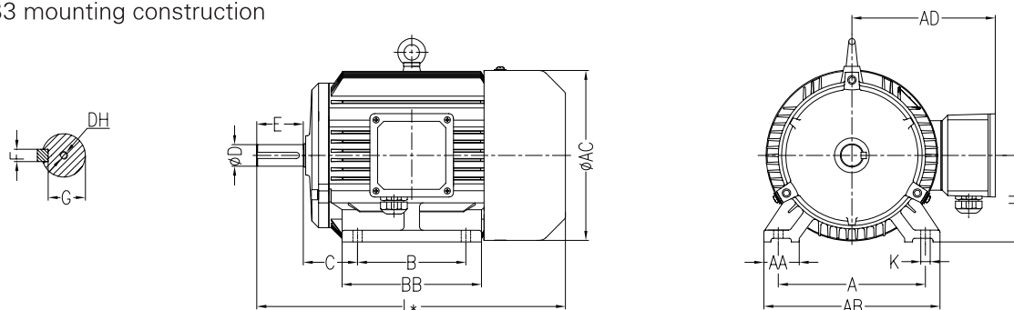
B3 mounting construction
